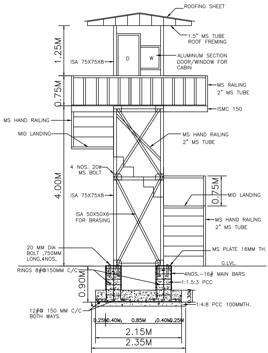
ELEVATION/SECTION
